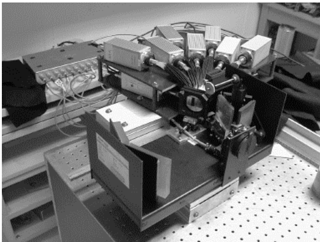
Figure 2.10 Photograph of the TS spectrometer. The 2-tier, stadium style layout of the LA-APD modules, the exit-plane fixture, the larger area mirror, the spectrometer shutter, and the APD power distribution box are visible.
