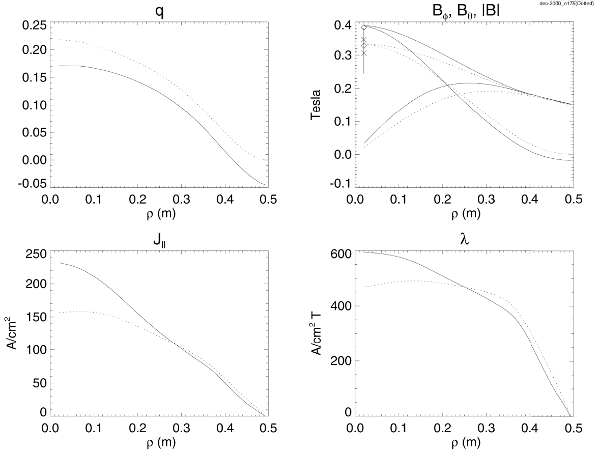
Figure 6.14 Comparison of equilibrium reconstructed profiles between Standard (solid) and Non-Reversed plasmas (dotted) shows a much flatter q -profile.
