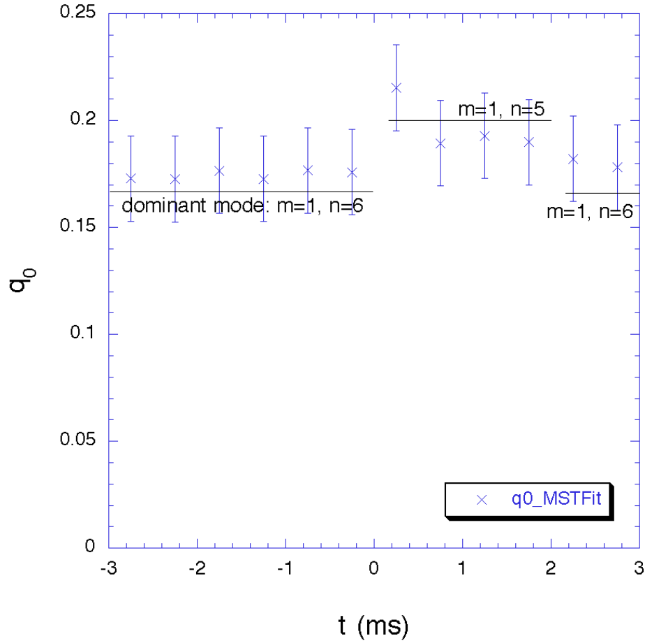
Figure 3.23 The on-axis value of q calculated from MSTFit should be high enough that the resonant surface of the observed, dominant magnetic mode is in the plasma.
