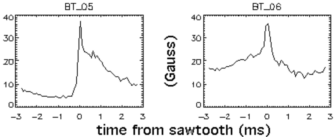
Figure 3.22 Time evolution of the n=5 and n=6 toroidal mode fluctuation amplitudes for a Standard plasma.
