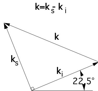
Figure 2.2 Wave vector diagram for Thomson scattering in the MST ruby laser system.
