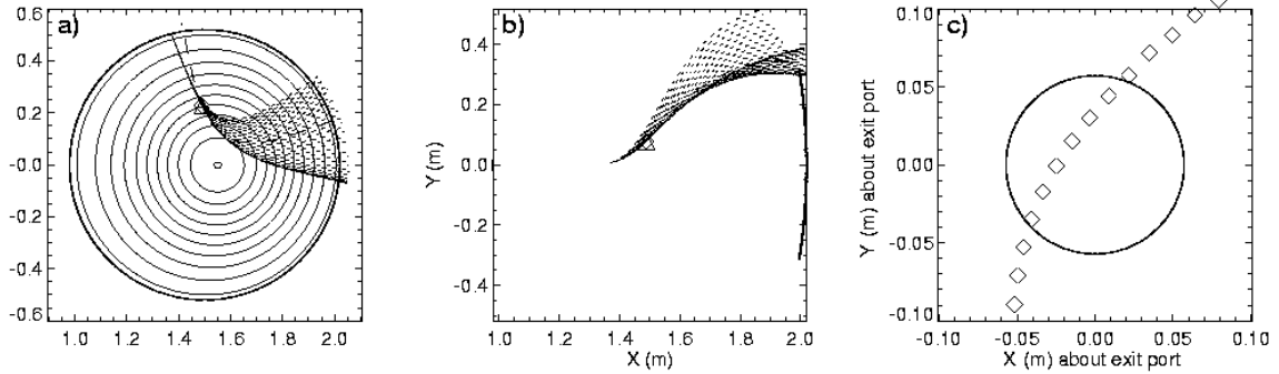
Figure 3.21 Trajectories of primary and secondary beam ions shown from a) a poloidal cross-section, and b) above, some of which c) intersect the energy analyzer entrance. Figure courtesy of Jay Anderson.
