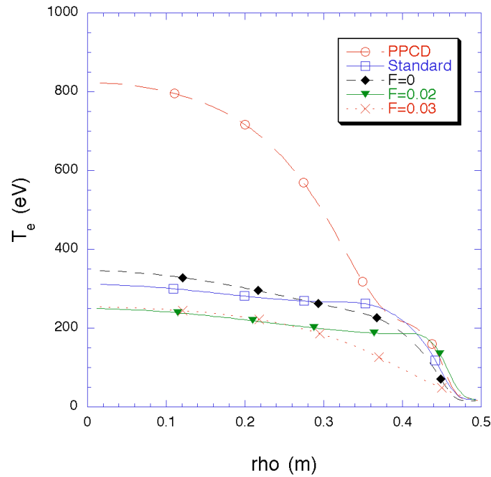
Figure 6.6 The electron temperature profile away from the nearest sawtooth crash.
