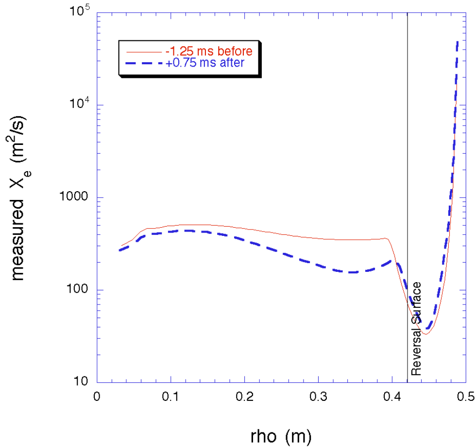
Figure 4.9 Measured electron thermal conductivity profiles at -1.25 ms (solid) and +0.75 ms (dashed) in Standard plasmas.
