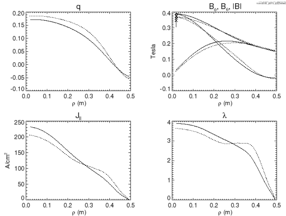
Figure 3.25 Current profile change in Standard plasmas from -1.75 ms (solid) before the crash to +0.75 ms (dotted) after the crash.
