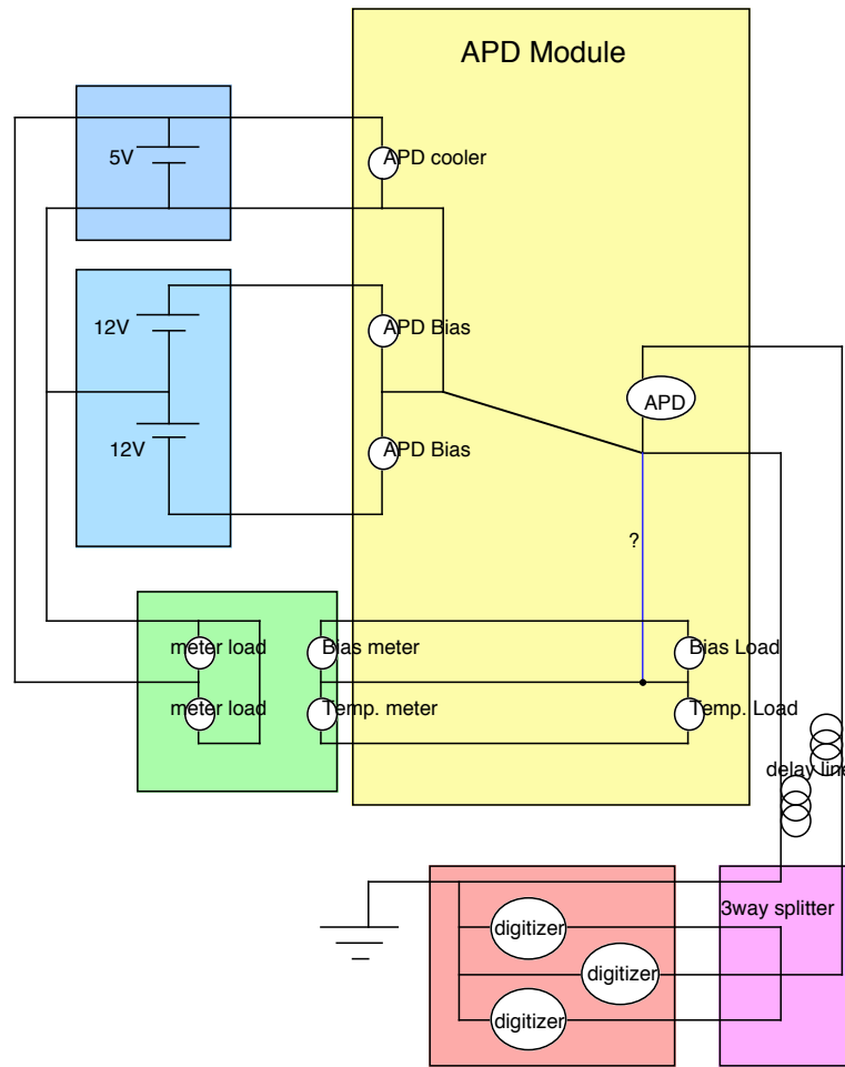
Figure 2.12 Circuit schematic of the LA-APD module system. Eleven modules are connected in parallel in this fashion, though only one is shown.
