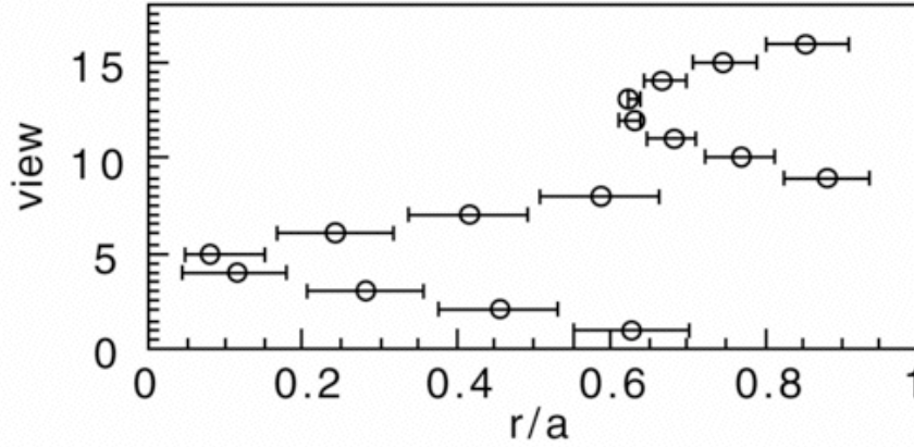
Figure 2.7 Geometrical coverage of ruby laser Thomson scattering views. Error bars indicate radial range (in r/a space) of scattering volume on each view.
