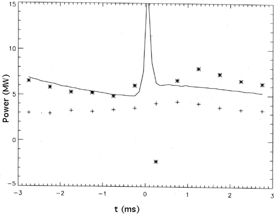
Figure 4.1 Comparison of the calculated Ohmic input power at the edge from the R -model (*) and from finite time-slice MSTFit (solid line). For comparison, the value of \int j^2 from MSTFit integrated over the volume is also shown (+) with flat Z_{\text{eff}}(r)=2 .
