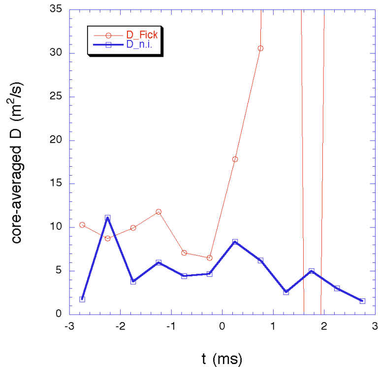
Figure 4.16 Core-averaged values of the electron diffusivity for Standard plasmas.
