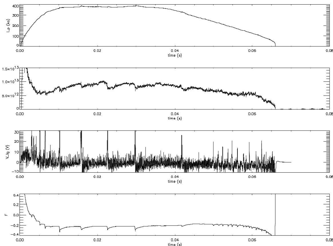
Figure 3.1 Shot 69 from November 13 th , 2000 showing the presence of sawteeth in a Standard MST plasma.
