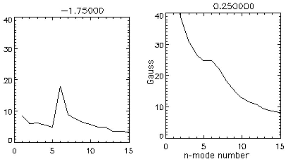
Figure 3.27 Sample n-spectra of the toroidal fluctuation amplitude at -1.75 ms and +0.25 ms. The dramatic increase of low-n fluctuations at the sawtooth is associated with m=0 activity.
