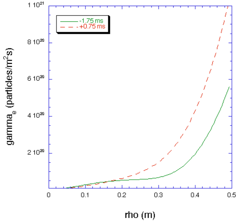
Figure 4.5 Measured electron flux profile at -1.75 ms and +0.75 ms relative to the sawtooth crash in Standard discharges.
