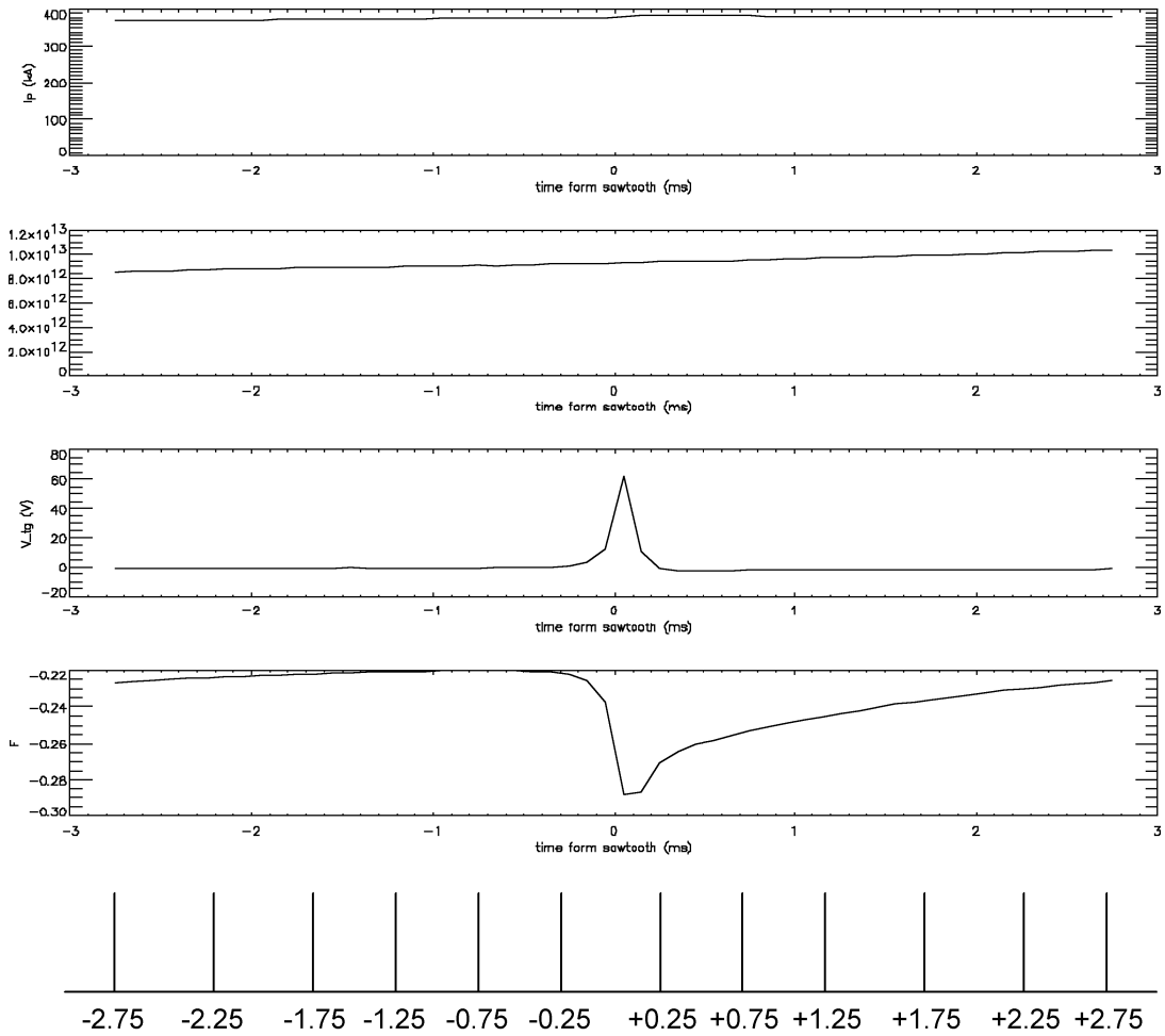
Figure 3.2 400 shot ensemble with respect to sawtooth crashes in “Standard” MST plasmas. The scale at the bottom shows the center locations of 0.5 ms time bins that are used in the following analysis.
