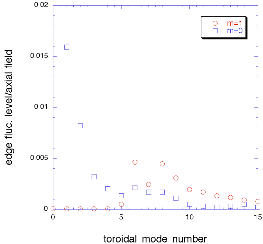
Figure 5.4 The n -spectra of m=0 and m=1 modes in the edge of the DEBS simulation is qualitatively similar to the spectra of Standard MST plasmas (Figure 3.29).
