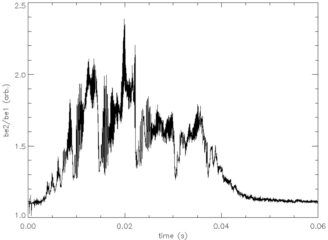
Figure 3.4 The ratio of two thin-filter (Beryllium) soft x-ray signals gives an indication of the level of temperature fluctuations in a Standard shot (Shot 17, 30-Mar-2001).
