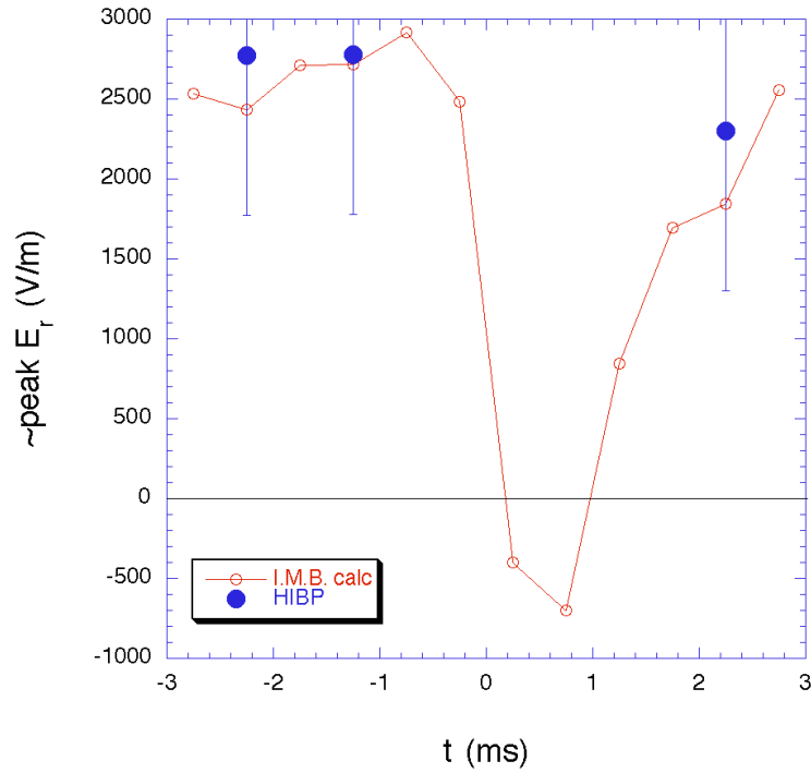
Figure 3.34 The mid-radius (~peak value) of the radial electric field as it evolves over the sawtooth cycle in Standard plasmas.
