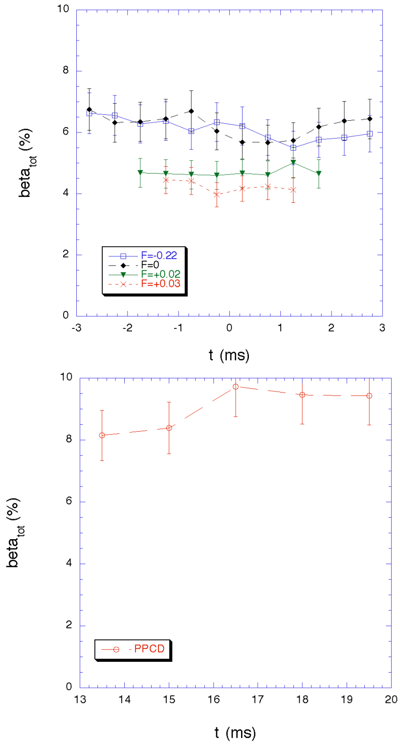
Figure 6.19 Total \beta over a sawtooth cycle for -0.22 < F < +0.03 plasmas, and during PPCD.
