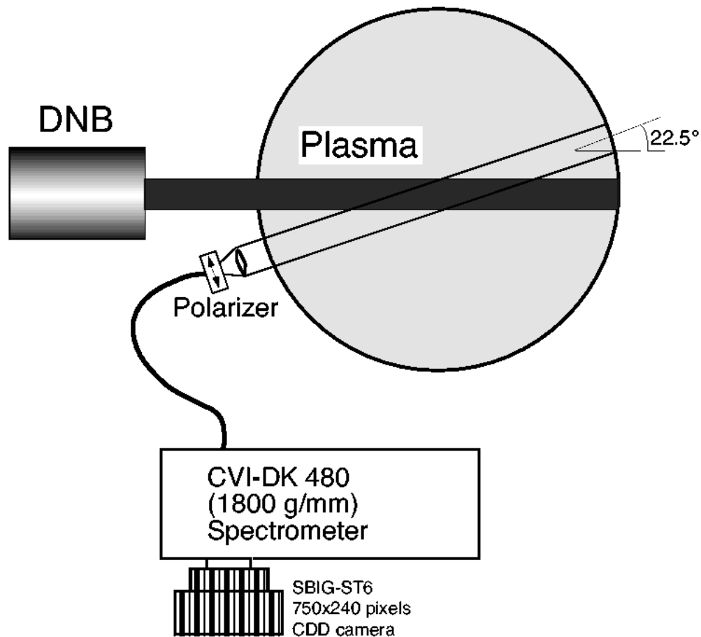
Figure 3.17 The MST motional Stark Effect diagnostic setup, courtesy of Jay Anderson. A diagnostic neutral beam, fired radially into the plasma experiences a changing magnetic field, because the equilibrium toroidal field peaks on-axis. The changing magnetic field appears to the neutral atoms as an electric field, which Stark-splits the lines of the neutral emission spectra. Measuring the spectral width of the Stark manifold then yields the magnetic field.
