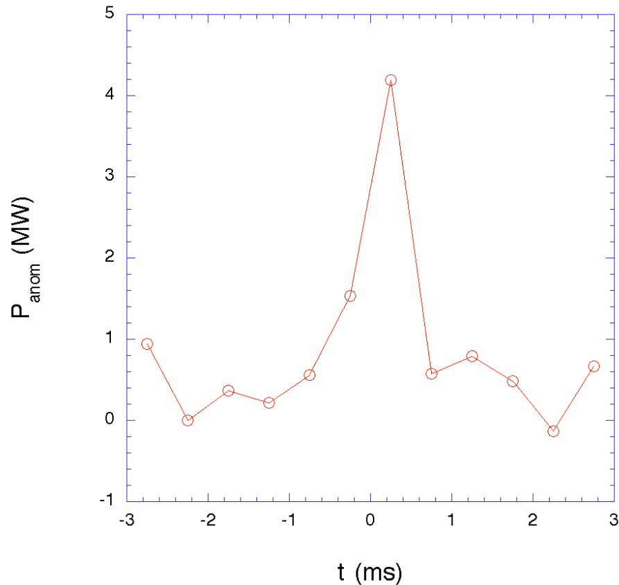
Figure 5.11 Anomalous power required if the ions have a 10 ms energy confinement time.
