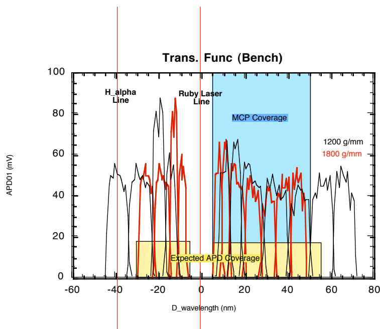
Figure 2.13 Bench measured instrument transfer function for the TS spectrometer with APD modules for both the 1200 g/mm and 1800 g/mm gratings. Also shown is the extent of the region previously covered by the MCP in the 1200 g/mm configuration, as well as the location of the H _{\alpha} Balmer line.
