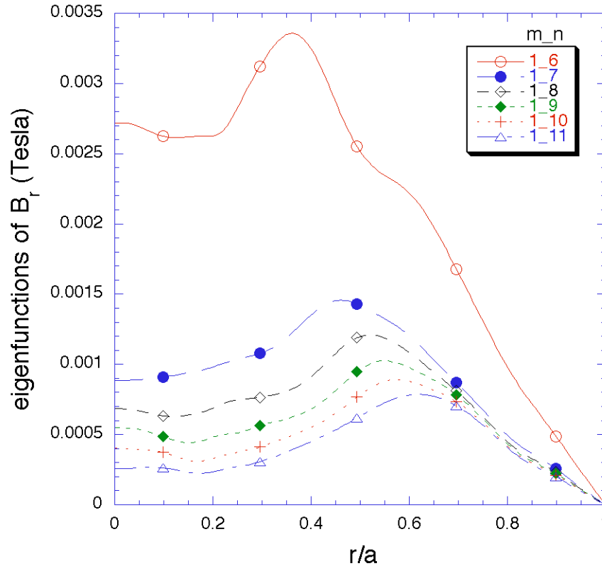
Figure 5.5 Radial fluctuation eigenfunctions as calculated by DEBS, scaled by the measured fluctuation amplitudes at the wall.
