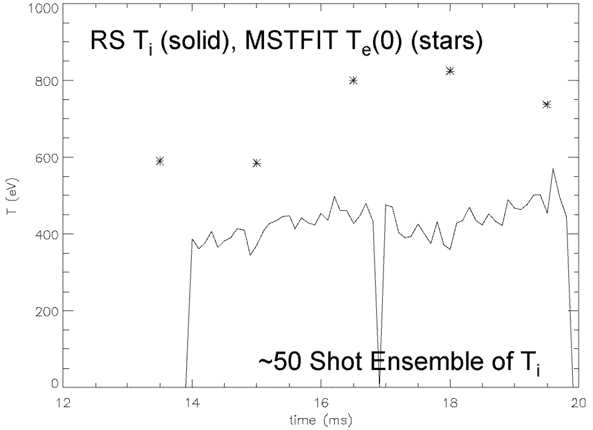
Figure 6.16 Electron and ion temperature evolution during PPCD discharges.
