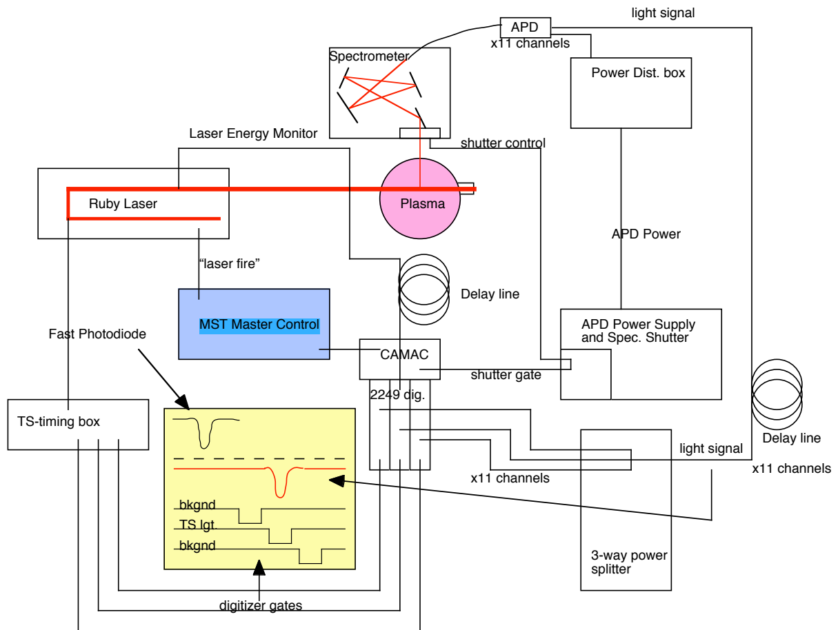
Figure 2.11 Schematic overview of the ruby laser TS system.
