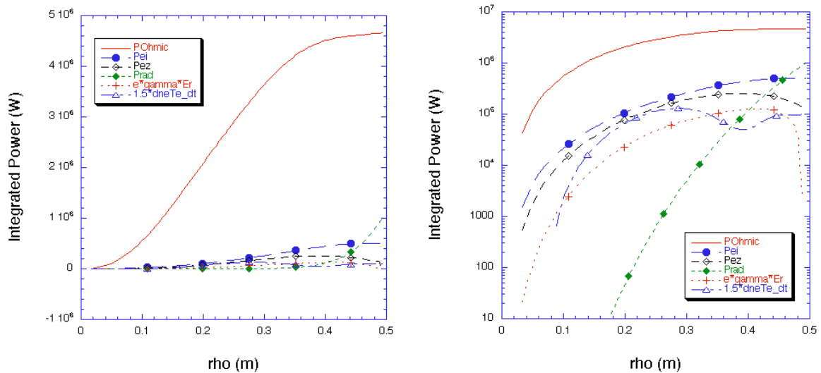
Figure 4.7 The electron energy budget at -1.75 ms in the sawtooth cycle of Standard plasmas on linear and logarithmic scales (to show detail).
