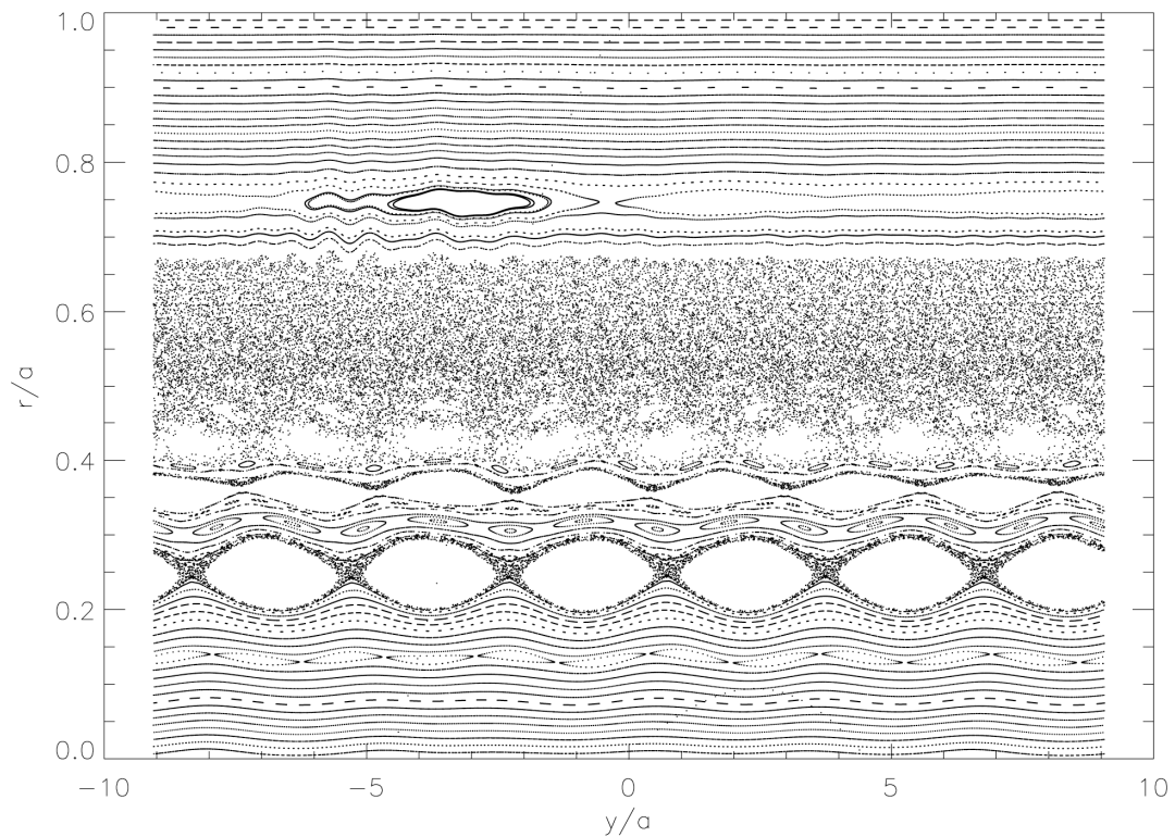
Figure 5.7 Puncture plot of magnetic field lines in Standard plasmas between sawteeth from DEBS/MAL simulation. Figure courtesy of Ben Hudson.
