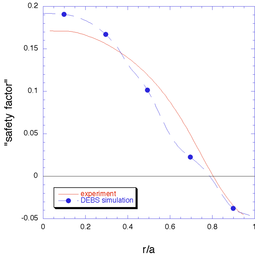
Figure 5.2 Comparison of the q -profiles from experiment (-1.75 ms before sawtooth crash) and from DEBS simulation at S \sim 10^6 .
