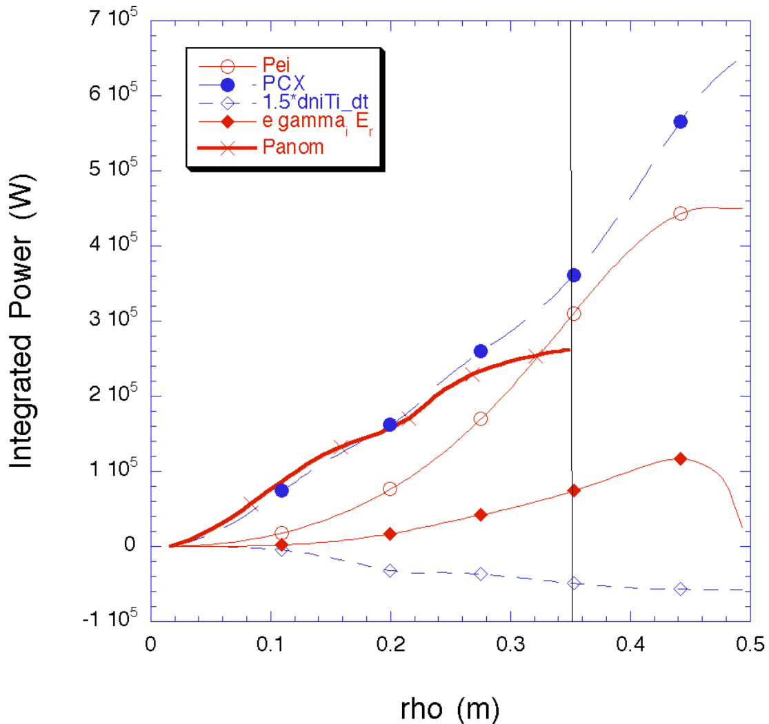
Figure 5.12 Ion energy budget at -1.75 ms in Standard plasmas.
