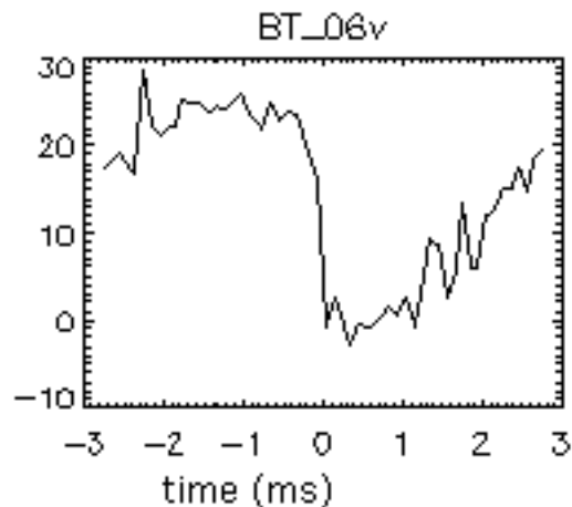
Figure 3.31 n=6 mode rotation velocity over the sawtooth crash during Standard plasmas. The y-axis is in km/s.
