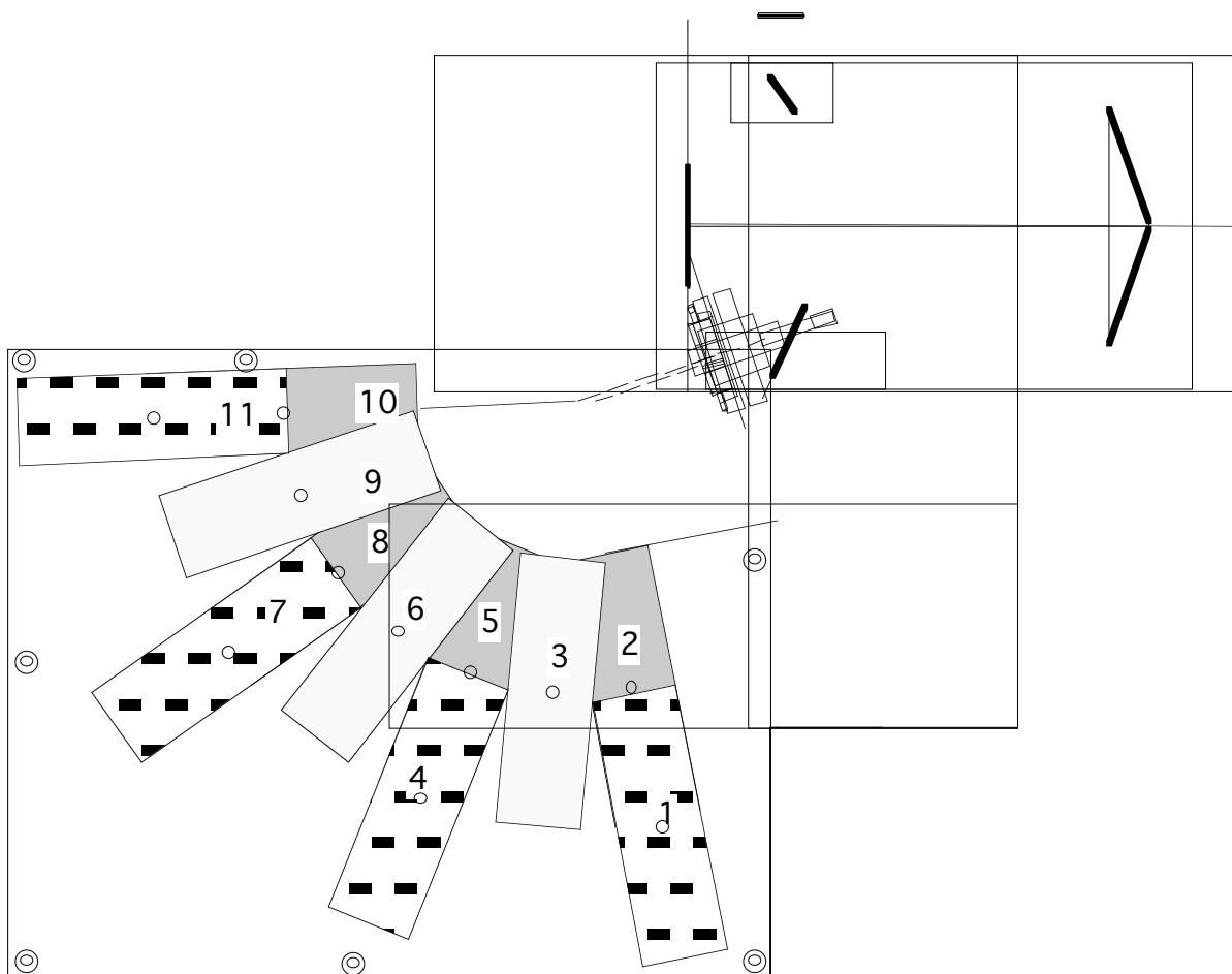
Figure 2.9 Schematic setup of the TS spectrometer, showing the 2-tier layout of the LA-APD modules.
