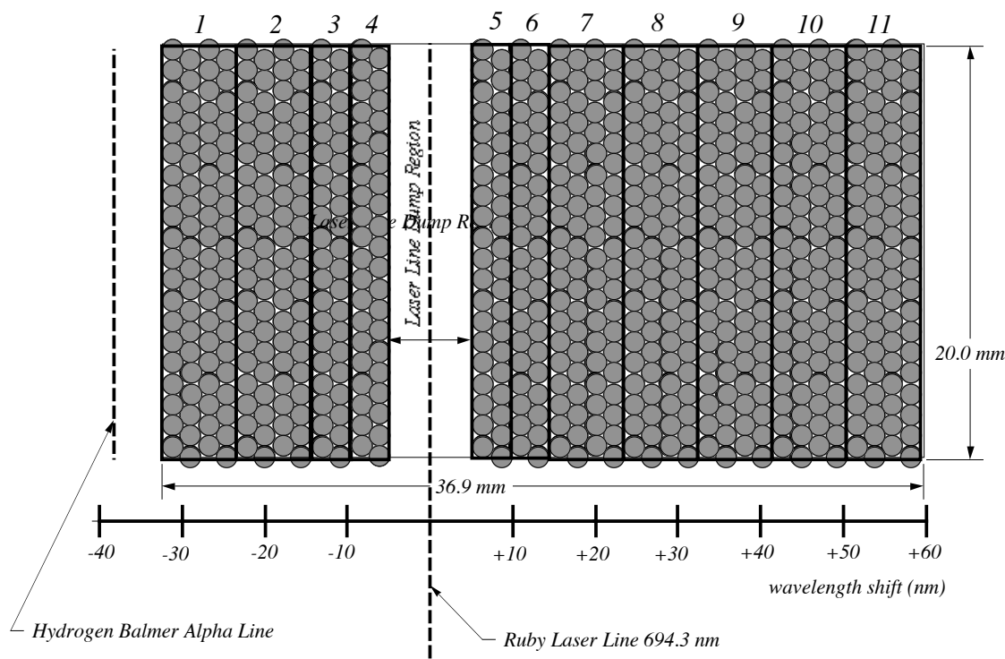
Figure 2.8 Schematic of the TS spectrometer exit-plane arrangement of fiber optics. Vertical groupings correspond to separate LA-APD modules.
