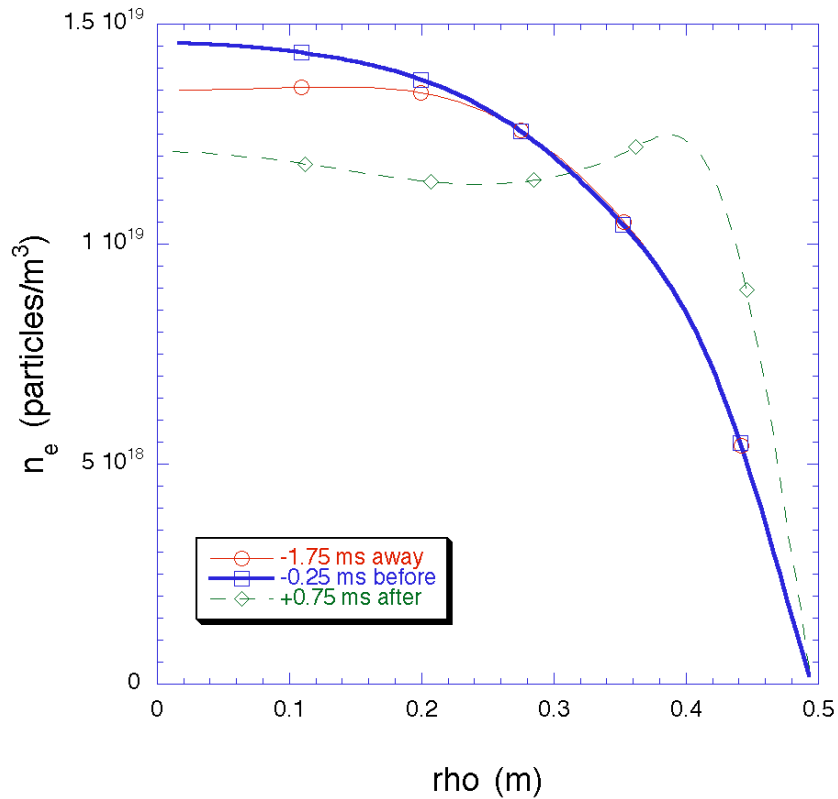
Figure 3.12 Select profiles of electron density during Standard plasma discharges.
