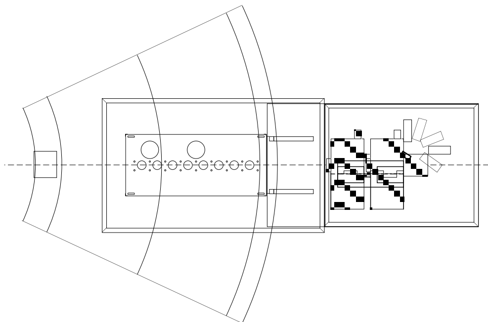
Figure 2.6 Top view of the ruby laser Thomson scattering system, showing a segment of the MST vacuum vessel. The spectrometer is shown in overlay at its two locations. The spectrometer is movable in order to reach the furthest inboard viewing locations with the fiber bundle. Only the top row of LA-APD modules is shown, in addition to the former location of the MCP detector.
