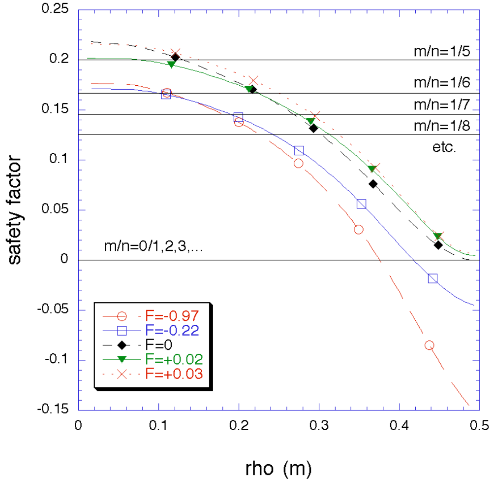
Figure 6.10 The safety factor profile away from the nearest sawtooth crash for all 5 plasma discharge types.
