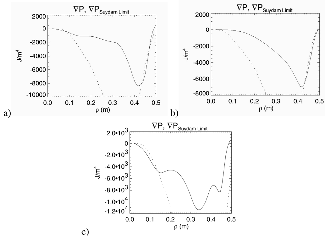
Figure 6.11 Comparison of the measured pressure gradient (solid line) with the calculated Suydam pressure gradient limit (dashed line) to ideal interchange modes: a) Standard ( F=-0.22 ) plasma (-1.75 ms), b) Non-Reversed ( F=0 ) plasma (-1.75 ms), c) PPCD plasma (18 ms).
