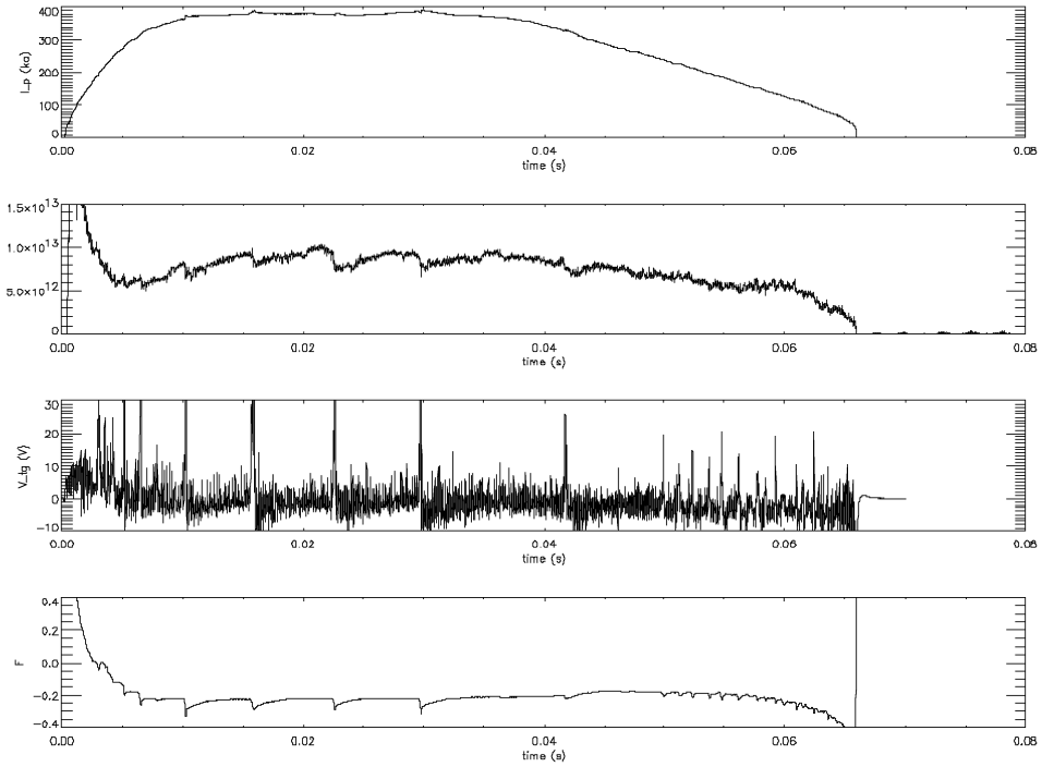
Figure 6.1 Shot 69 from November 13 th , 2000 showing a typical “Standard” MST plasma.
