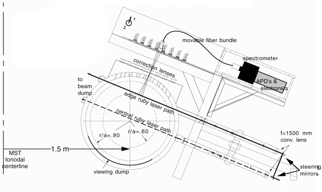
Figure 2.4 Side view of the ruby laser Thomson scattering system at 90 degrees toroidal of the Madison Symmetric Torus. To operate in “central” laser path mode, the lower steering mirror is removed along with the movable correction lenses.
