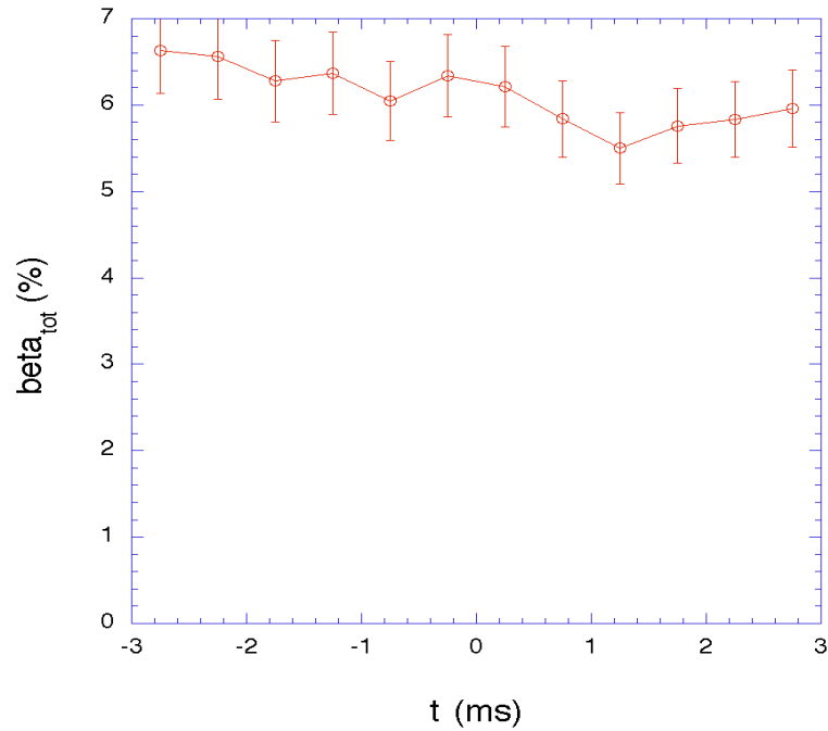
Figure 6.17 Total \beta over the sawtooth cycle for Standard plasmas.
