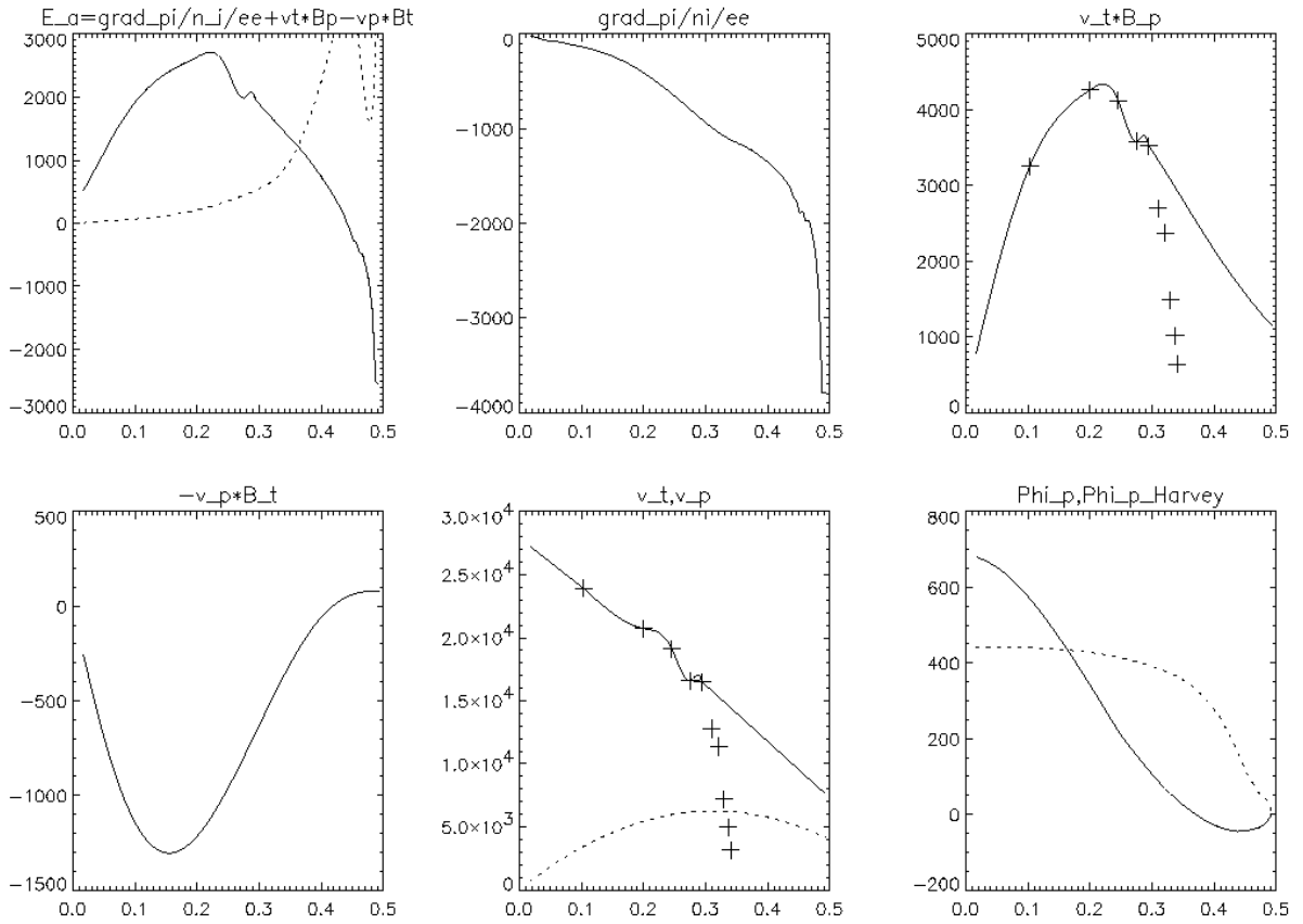
Figure 3.32 Radial electric field profile and the terms used in its calculation for a Standard plasma, -1.75 ms away from the sawtooth crash.
