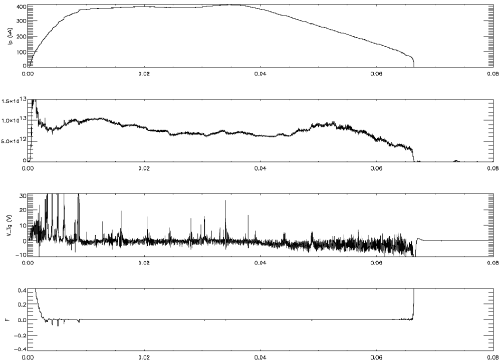
Figure 6.2 Shot 80 from March 30 th , 2001 showing a typical “Non-Reversed” MST plasma.
