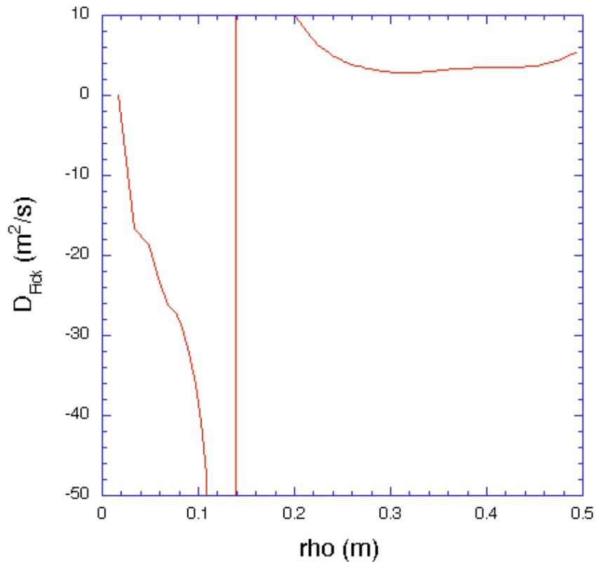
Figure 4.14 The electron diffusion coefficient derived from Fick's Law at -1.75 ms in Standard discharges.
