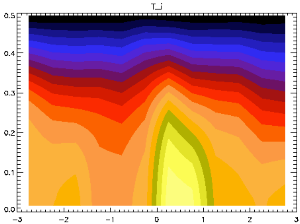
Figure 3.10 Surface and contour plots of the RS measured ion temperature profile evolution over the sawtooth cycle in Standard plasmas.
