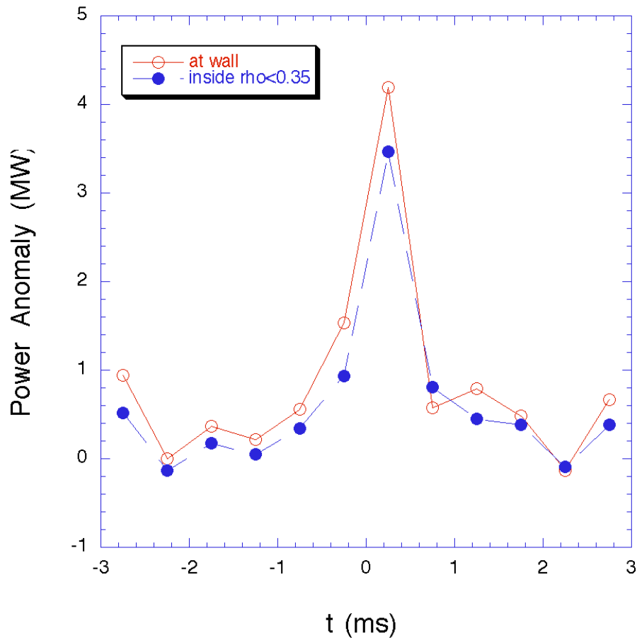
Figure 5.13 Comparison between core&mid-radius and whole plasma of the amount of expected anomalous ion heating.
