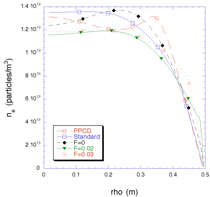
Figure 6.7 The electron density profile away from the nearest sawtooth crash.
