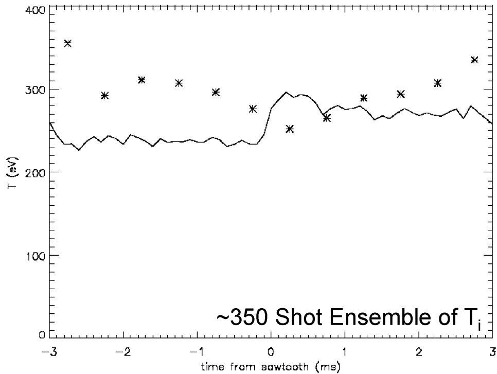
Figure 6.12 Anomalous ion heating at the sawtooth crash in Standard plasma, as measured by Rutherford scattering (solid), compared to the Thomson scattering measured electron temperature (stars.)
