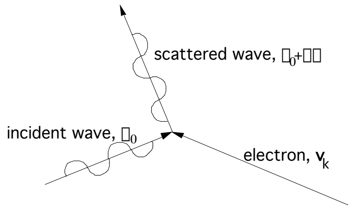
Figure 2.1 Thomson scattering of light from a moving electron.
