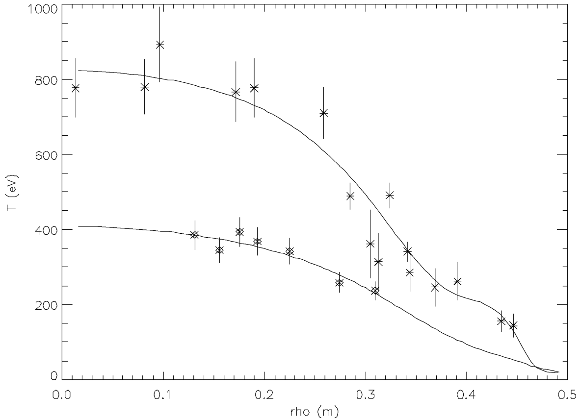
Figure 6.15 Electron and ion temperature profiles at 18 ms, during PPCD plasma discharges.
