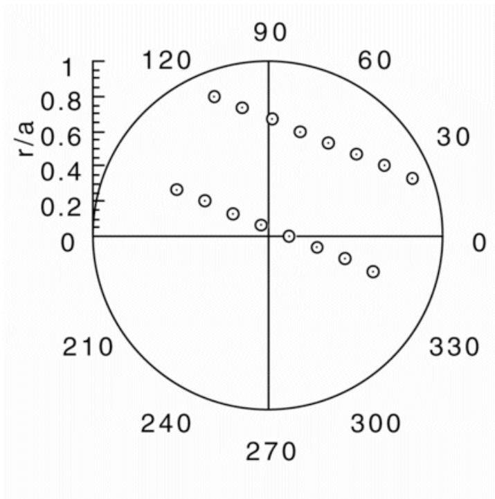
Figure 2.5 Geometrical location of Thomson scattering viewing centers for both the edge and central laser paths.
