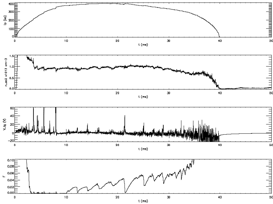
Figure 6.4 Shot 69 from April 2 nd , 2001 showing a typical “F= +0.03” MST plasma: a small increase in F leads to a rapid degradation of the plasma.
